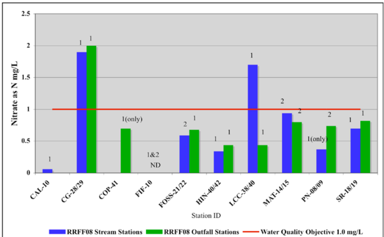
Figure 3.4: Nitrate as (N) concentrations by station
