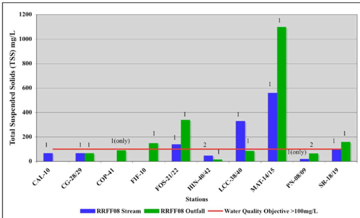
Figure 3.9: Total Suspended Solids (TSS) concentrations by station
