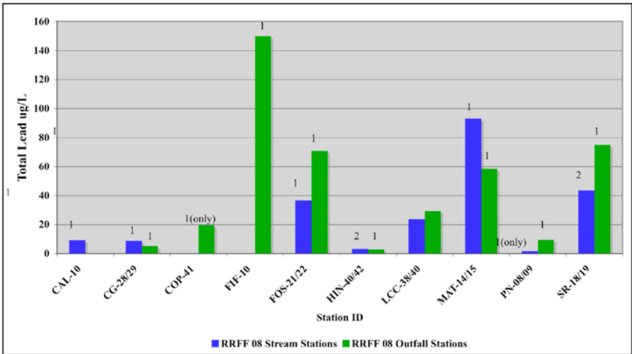
Figure 3.6: Total Lead concentrations by station
