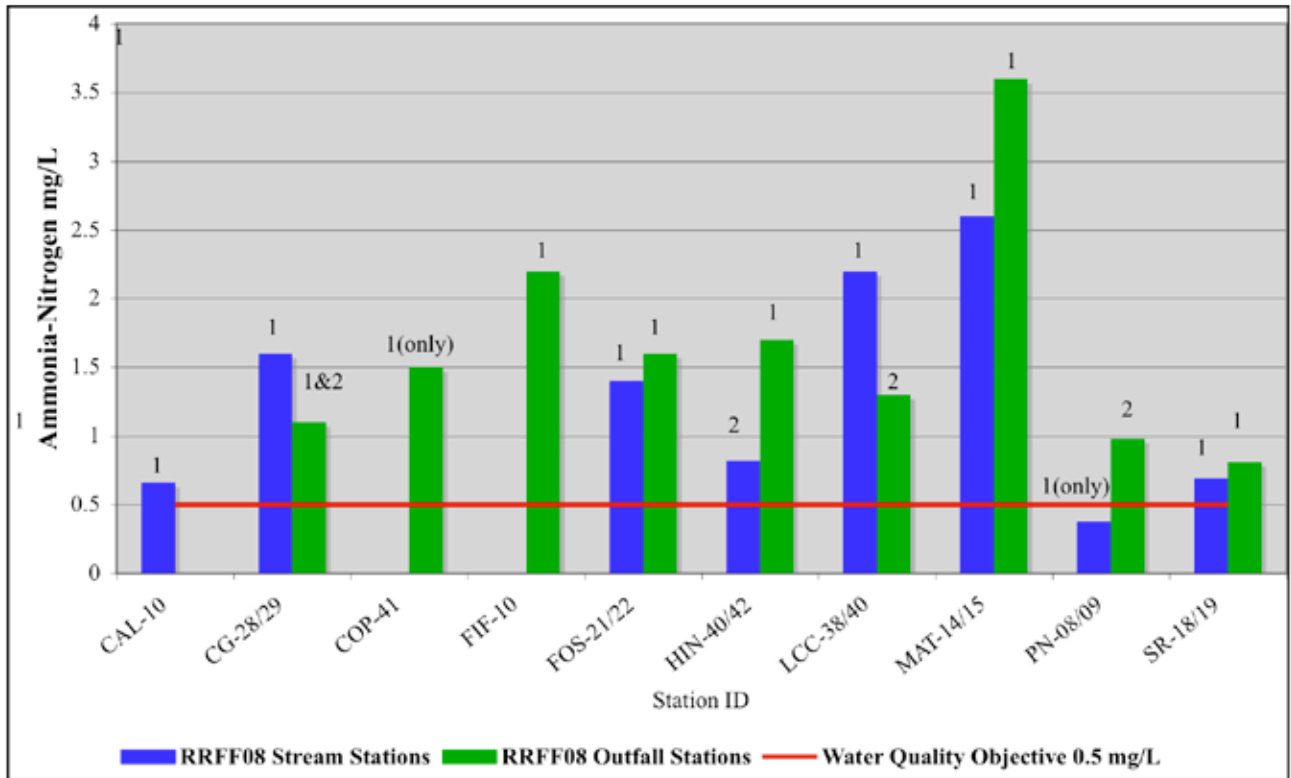
Figure 3.3: Ammonia-Nitrogen concentration by station
