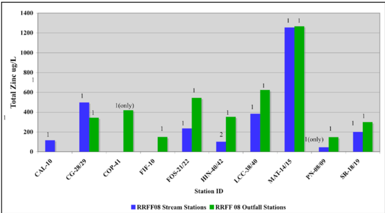
Figure 3.7: Total Zinc concentrations by station
