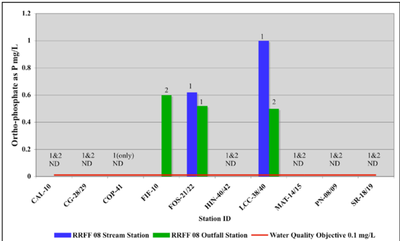
Figure3.5: Ortho-phosphate as (P) concentrations by station
